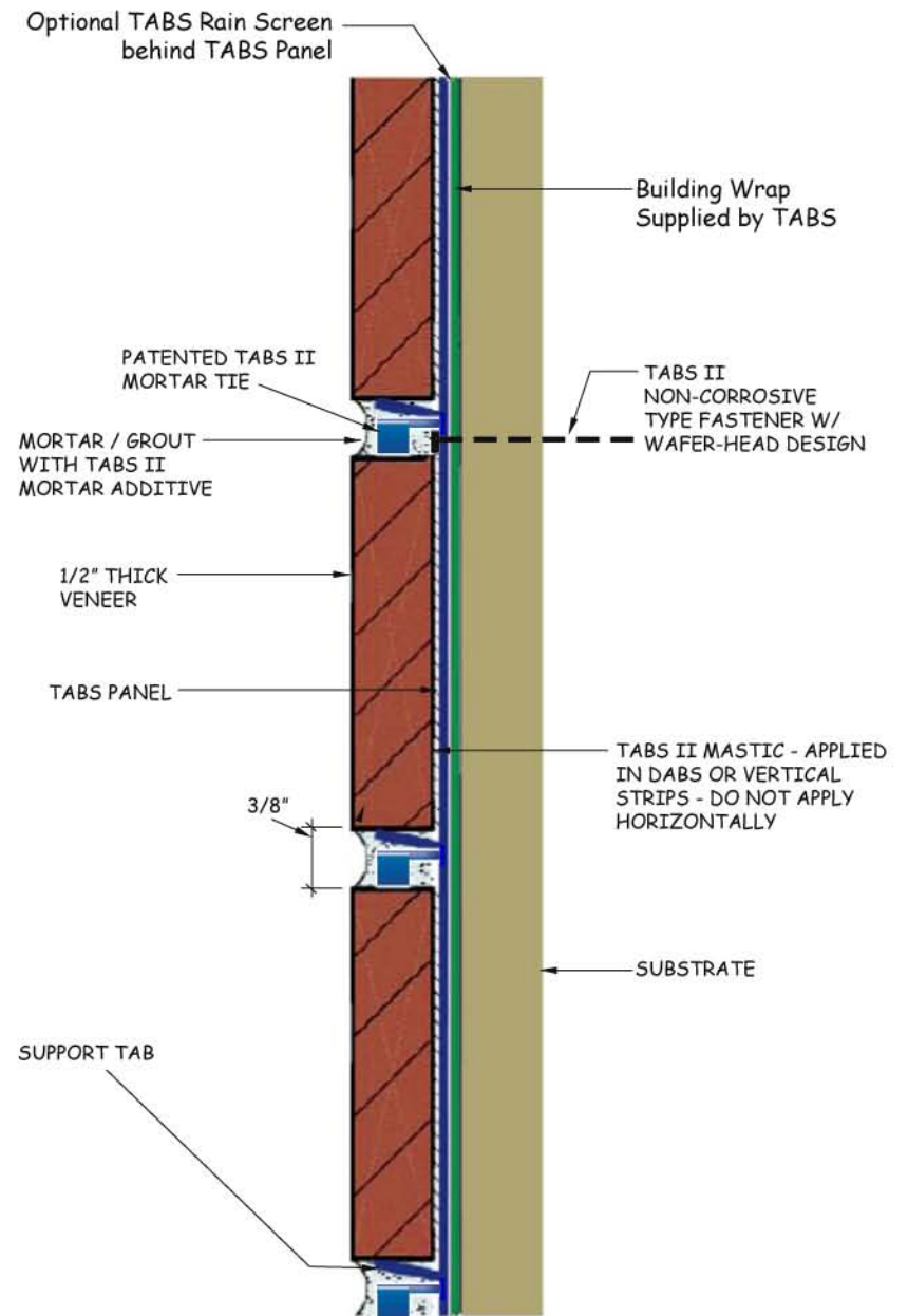
TYPICAL WALL DETAIL
